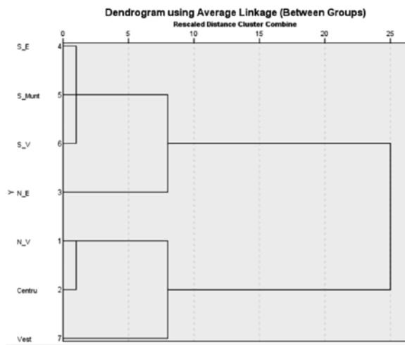
Figure 3. Dendrogram clustering all regions, except for Bucharest-Ilfov in 2007
