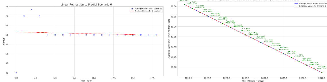
Picture 8-9: Predict a Scenario6 based with Linear Regression algorithm (Source: authors' own survey with Microsoft Excel and Python)
